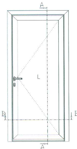
Όψη/Elevation
