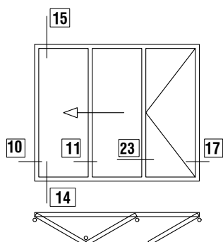
INWARDS OPENING 2 +1 3-PANELS FOLDING DOOR ΕΞΩ ΑΝΟΙΓΟΜΕΝΗ 2+1 3-ΦΥΛΛΗ ΦΥΣΟΥΝΑ
