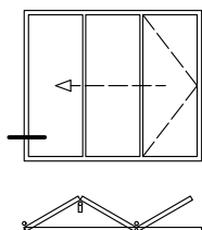
Position 1 Hinge side
