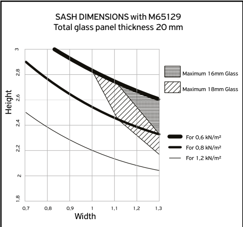
Max Dimensions – Wind load with aluminium reinforcement
