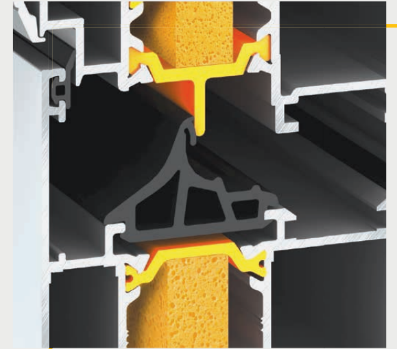
EPDM central gasket, which serves as the primary barrier between the window frame and the sash, helping to block air and water infiltration. This enhances the overall weatherproofing of the system, preventing the leaks.
