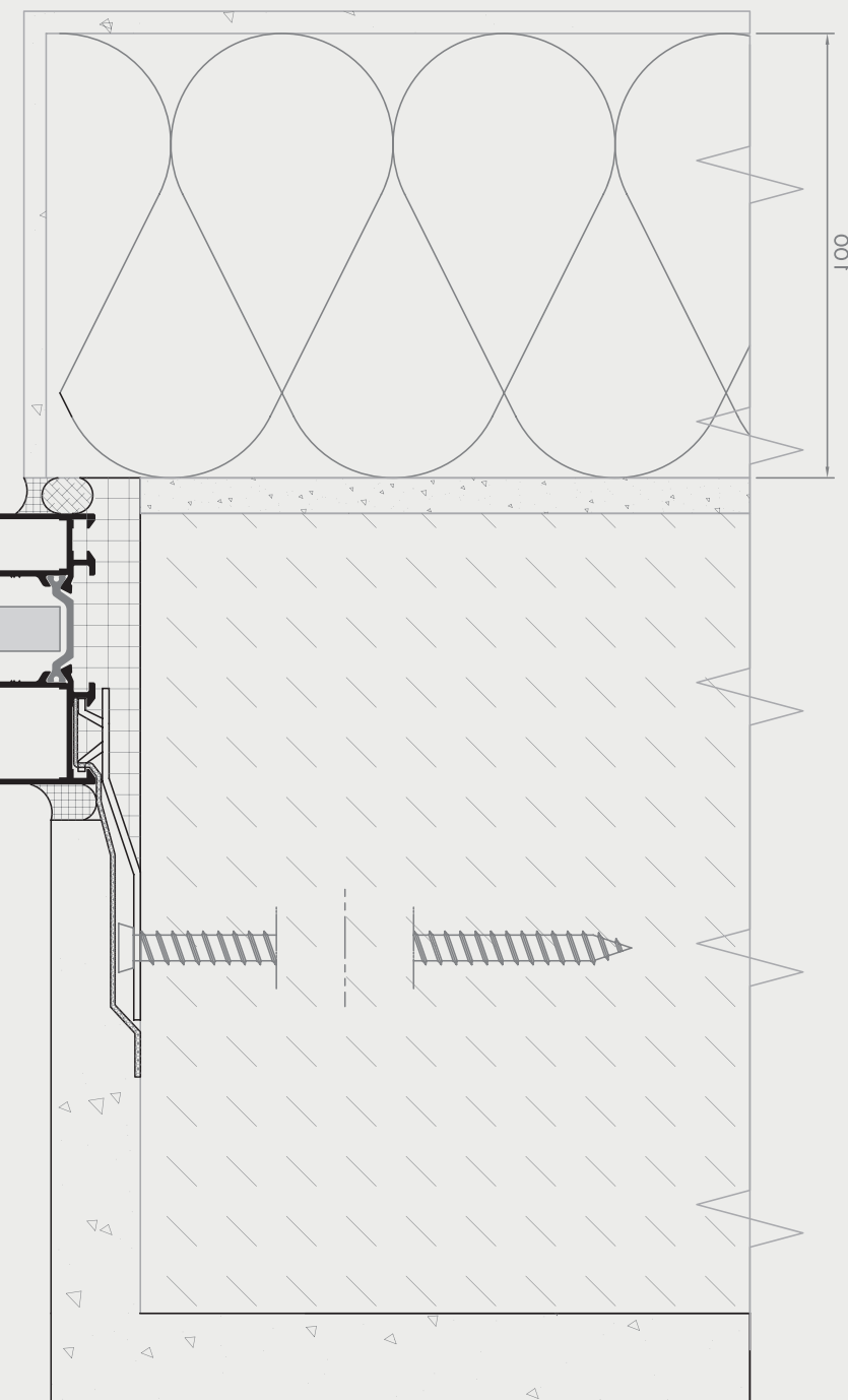
SIDE SECTION
