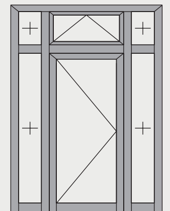
SINGLE LEAF DOOR WITH FANLIGHT AND FIXED LIGHTS
