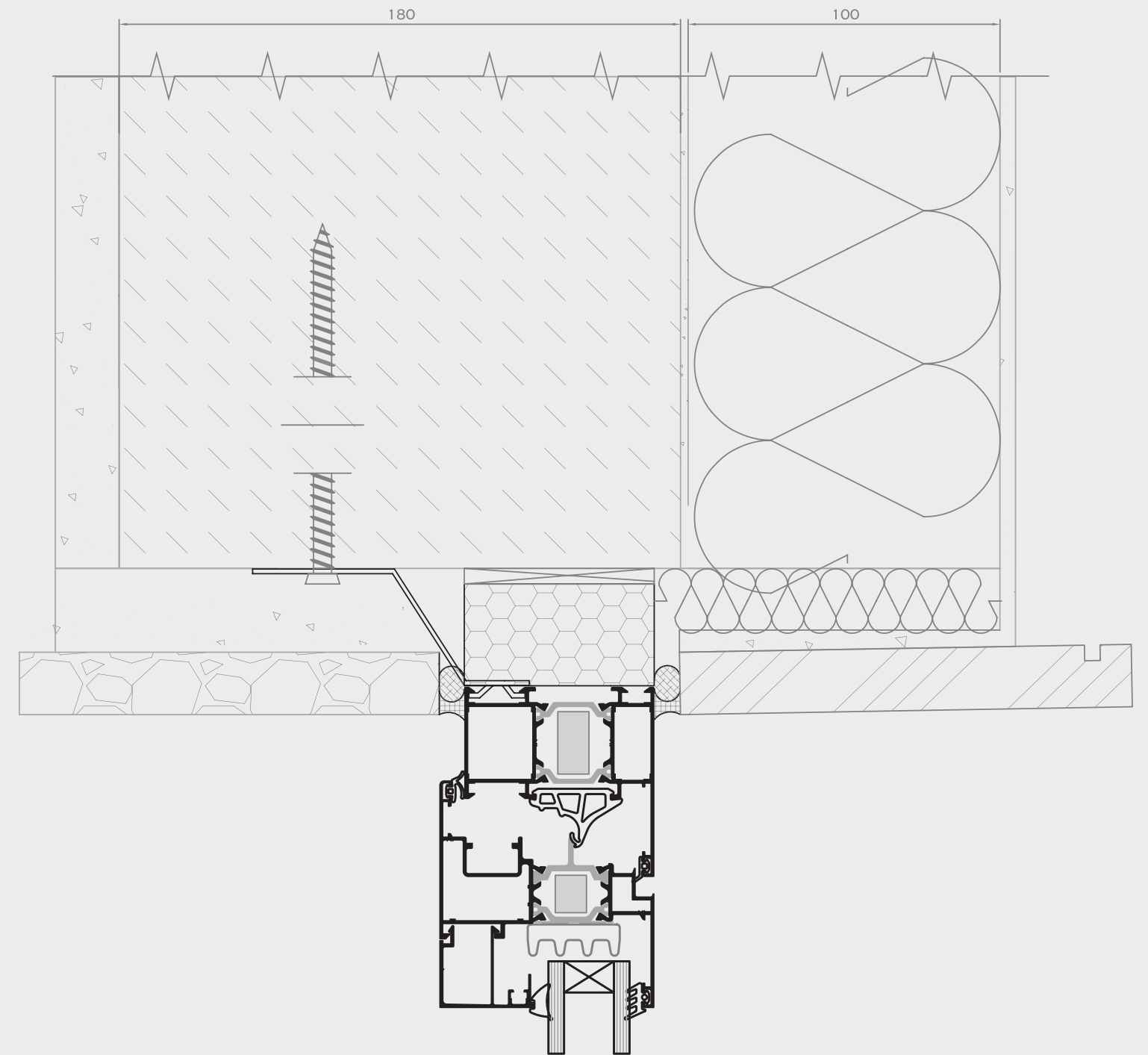
TOP SECTION
